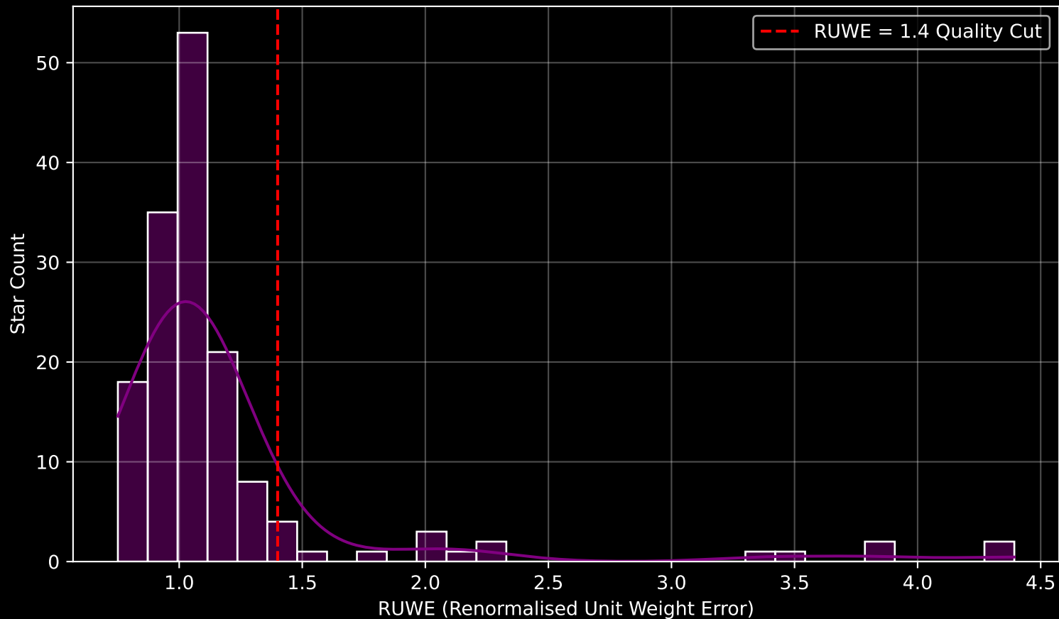
GAPOGEE DR17 Field [283-19-O_TESS] RUWE Distribution (n= 153)
