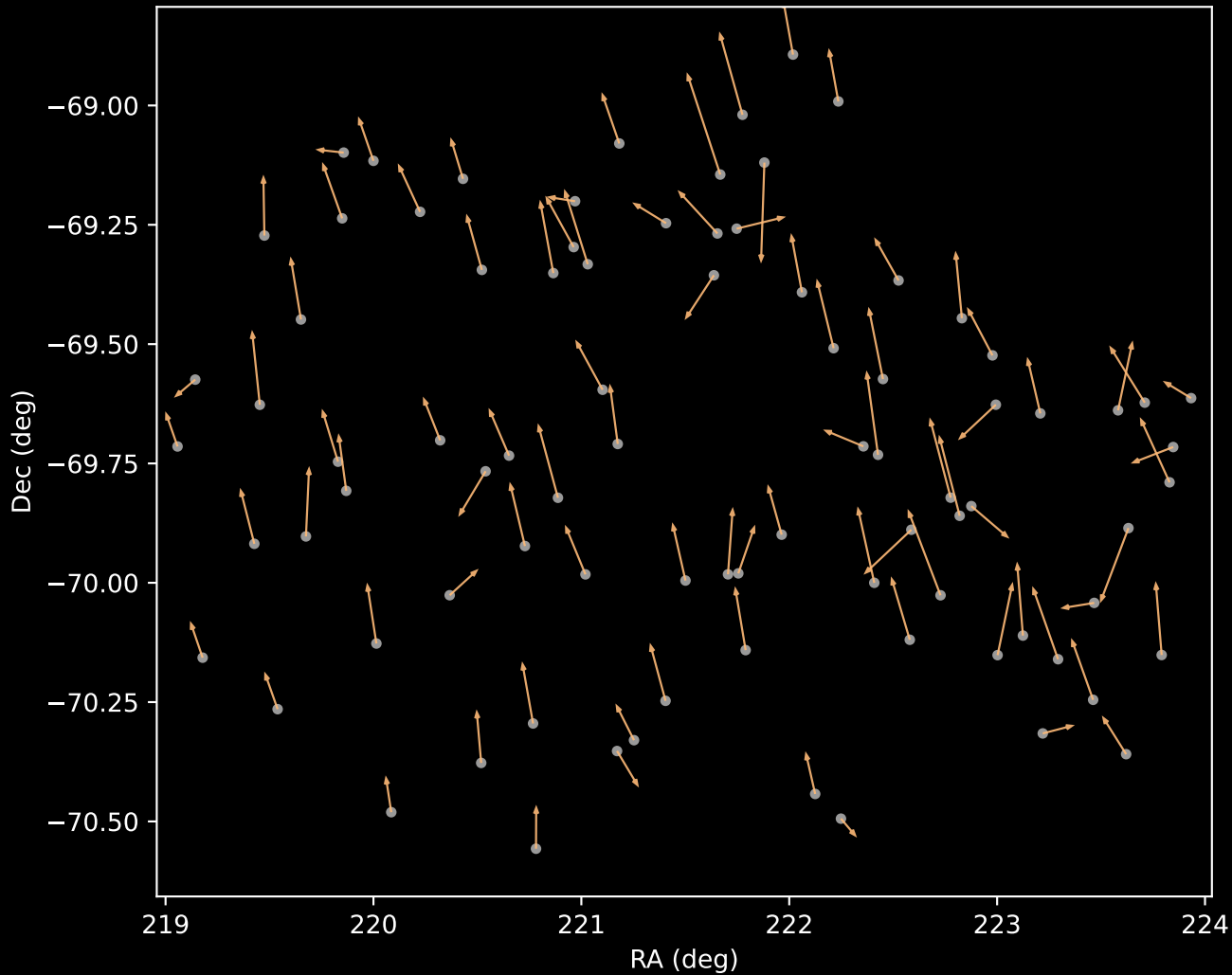
APOGEE DR17 Cluster 3 Proper Motion Vectors (n=86)
