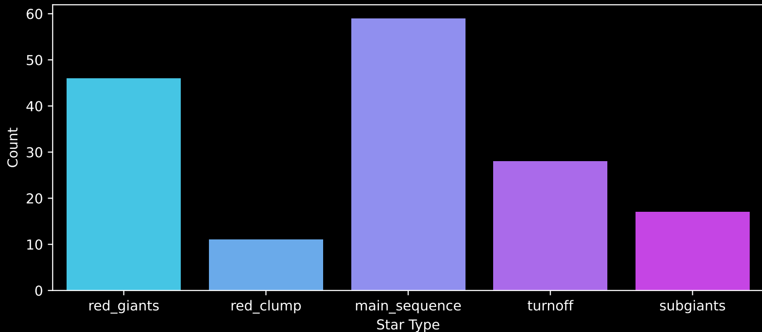
APOGEE DR17 Field: [283-19-O_TESS] Count plot of Star Type
